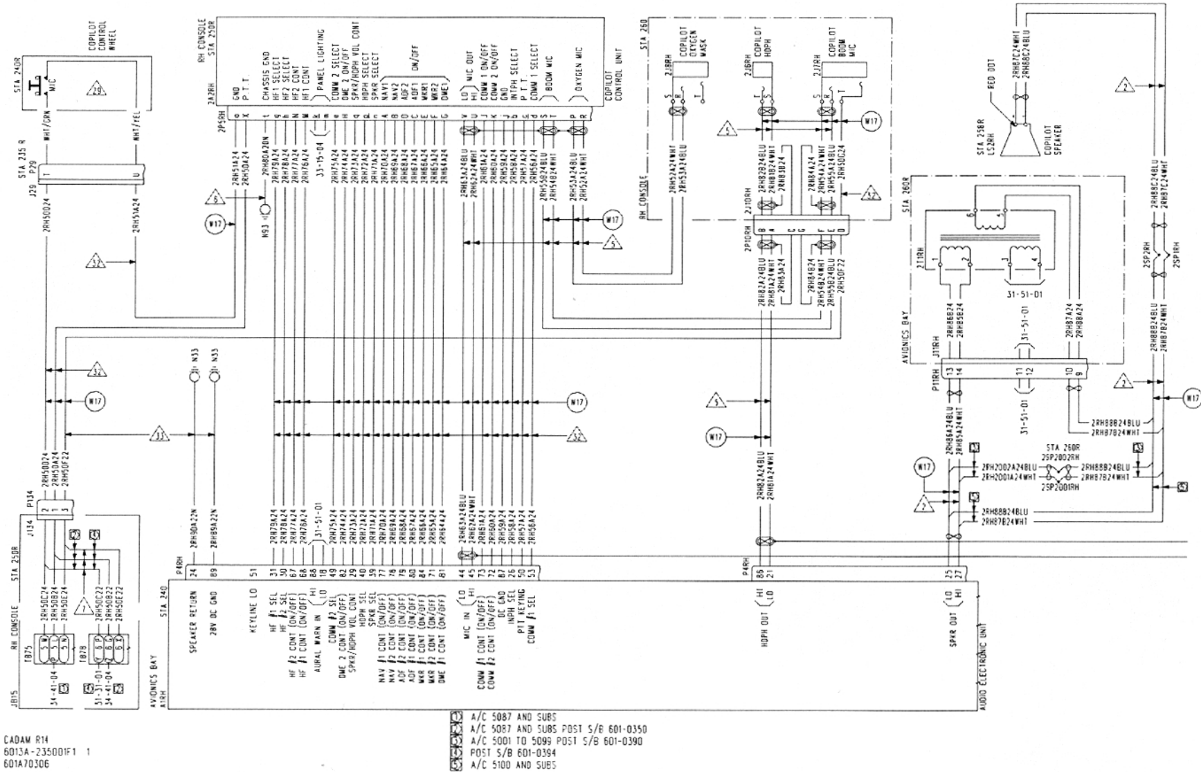
INTERCOM SYSTEM (DOT, FAA AND CAA CERTIFIED A/C) FIGURE 1 (SHEET 1)
