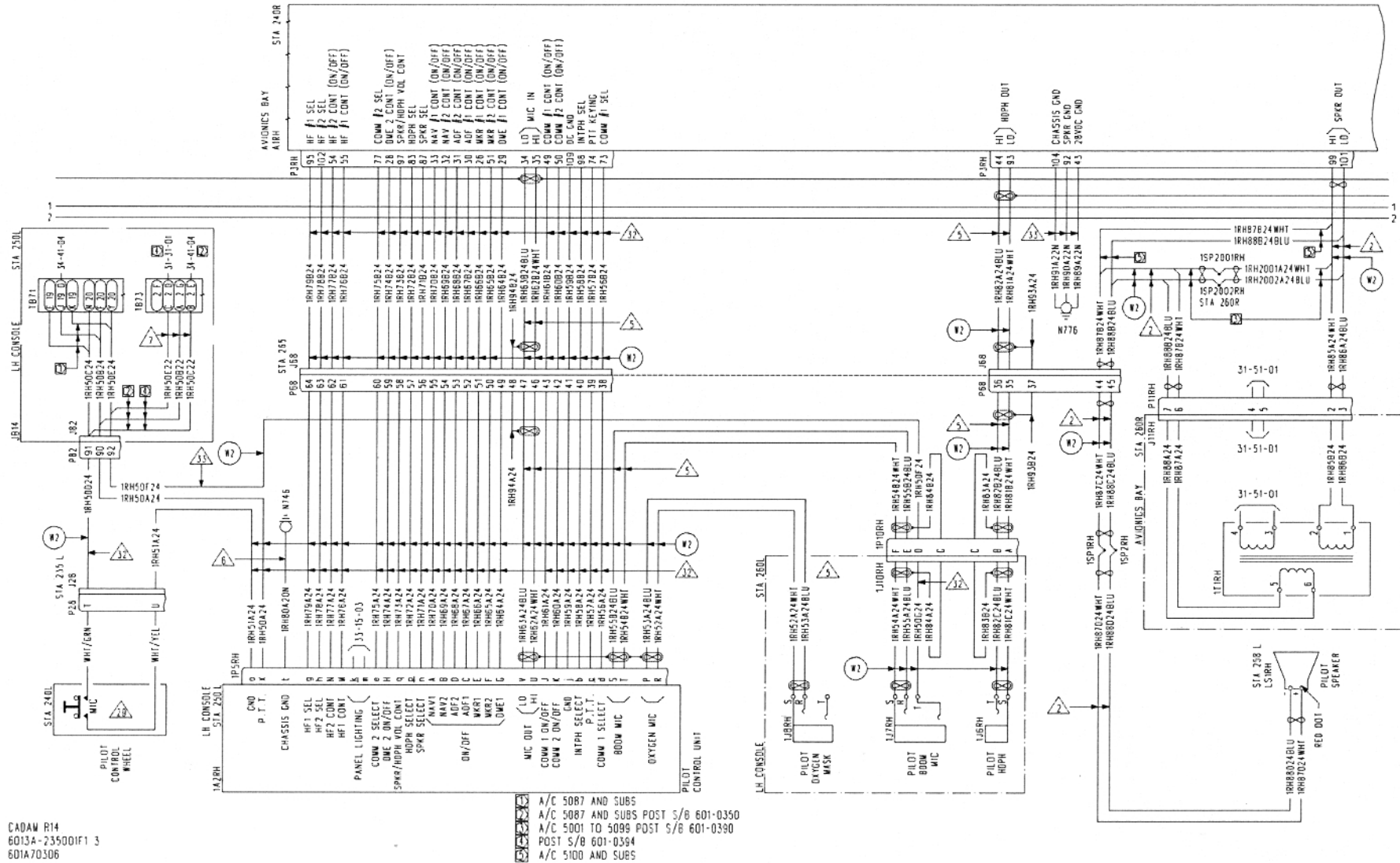
INTERCOM SYSTEM (DOT, FAA AND CAA CERTIFIED A/C) FIGURE 1 (SHEET 3)
